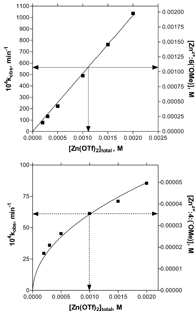
Figure 5. (a, top) k_{\text{obs}} for methanolysis of paraoxon as a function of [\text{Zn}(\text{OTf})_2]_{\text{total}} containing equimolar 6 and \text{NaOCH}_3 , T = 25^\circ\text{C} . \blacksquare represents the actual experimental rate constant (left axis). The solid line represents [\text{Zn}^{2+}:\text{6}(\text{OCH}_3)] (right axis) determined by Hyperquad fitting of titration data (see the Results, section d). The arrows are presented as a visual aid to connect the various species concentrations with the kinetic constant. (b, bottom) k_{\text{obs}} for the methanolysis of paraoxon as a function of [\text{Zn}(\text{OTf})_2]_{\text{total}} containing equimolar 4 and 0.5 equiv of \text{NaOCH}_3 , T = 25^\circ\text{C} . \blacksquare represents the actual experimental rate constant (left axis). The solid line represents [\text{Zn}^{2+}:\text{4}(\text{OCH}_3)] (right axis) determined by Hyperquad fitting of the titration data (see the Results, section d). The arrows are presented as a visual aid to connect the various species concentrations with the kinetic constant.
