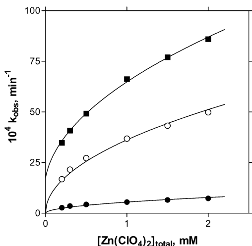
Figure 2. k_{\text{obs}} for the methanolysis of 3 (●), 1 (○) and p -nitrophenyl acetate (■) vs [Zn(ClO 4 ) 2 ] at a constant [Zn 2+ (-OCH 3 )]/[Zn 2+ ] total ratio of 0.3, T = 25\text{ }^{\circ}\text{C} . Lines through the data are calculated on the basis of eq 2. Note the nonzero intercept for the most reactive substrate, p -nitrophenyl acetate, attributable to the background reaction, which at \text{pH } 10.00 is k_{\text{obs}} = 2.2 \times 10^{-3}\text{ min}^{-1} .
