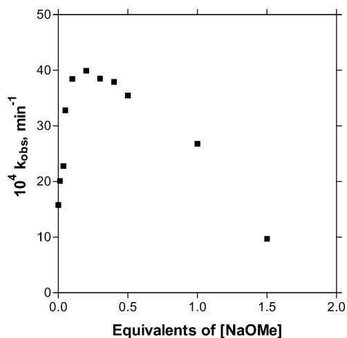
Figure 1. k_{\text{obs}} for the methanolysis of 1 vs added NaOCH 3 in the presence of 1 mM Zn(OTf) 2 , T = 25\text{ }^{\circ}\text{C} .
