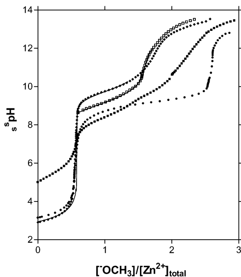
Figure 7. Potentiometric titration of 2 mM \text{Zn}(\text{OTf})_2 with no added ligand ( \bullet ), with 2 mM 4 ( \blacklozenge ), with 2 mM 5 ( \blacksquare ), and with 2 mM 6 ( \square ) with 1.2 mM added \text{HClO}_4 . Lines through the titration curves with 4 and 6 were derived from Hyperquad fitting of the data to models given in the Results, section d.
